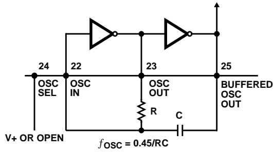
FIGURE 10. RC OSCILLATOR
