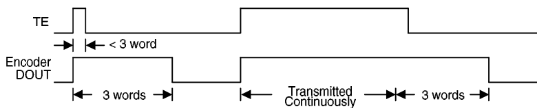
Transmission timing
