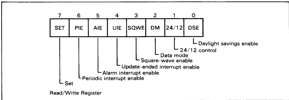
Figure 6. Register B
