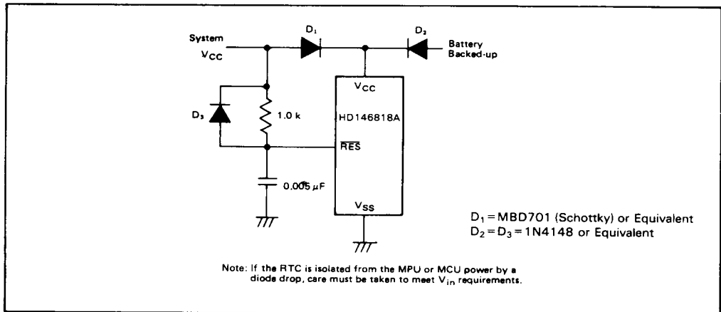
Figure 2. Typical Powerup Delay Circuit for RES
