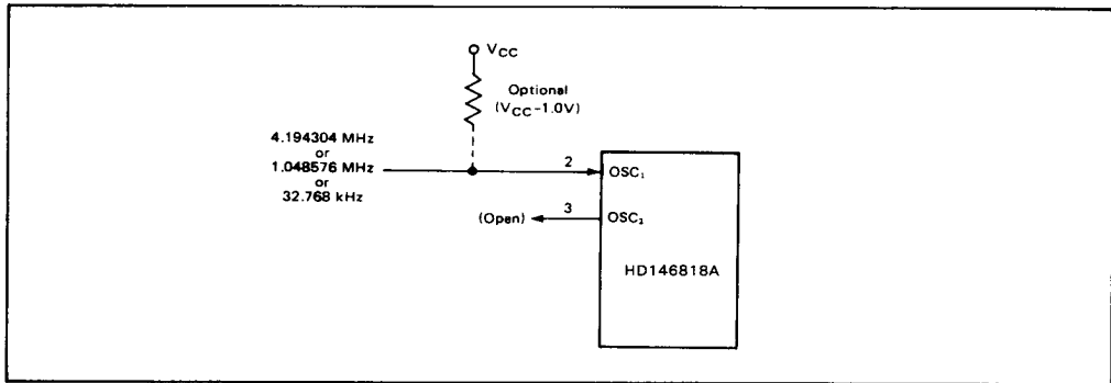
Figure 1. External Time-Base Connection
