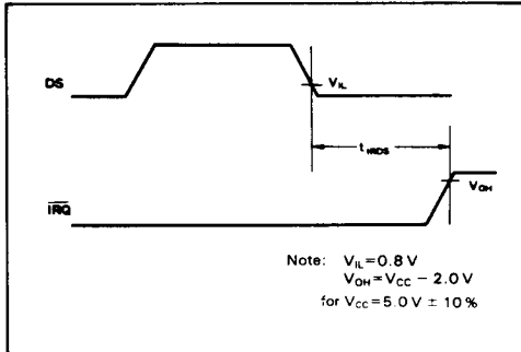
Figure 22. \overline{\text{IRO}} Release Delay (from DS)
