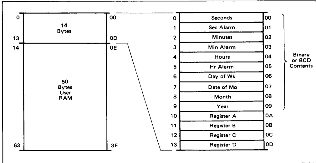
Figure 9. Address Map
