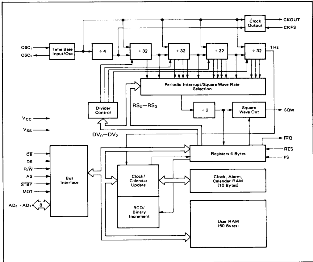
Figure 4. Block Diagram
