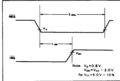
Figure 23. \overline{\text{IRO}} Release Delay (from RES)
