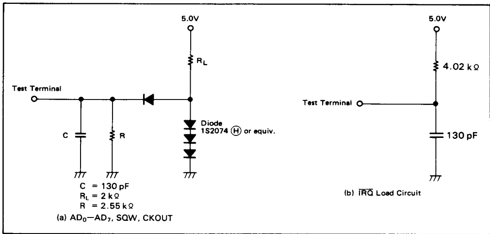
Figure 26. Test Load
