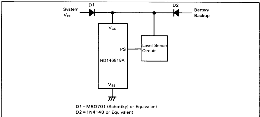
Figure 3. Typical Powerup Delay Circuit for Power Sense
